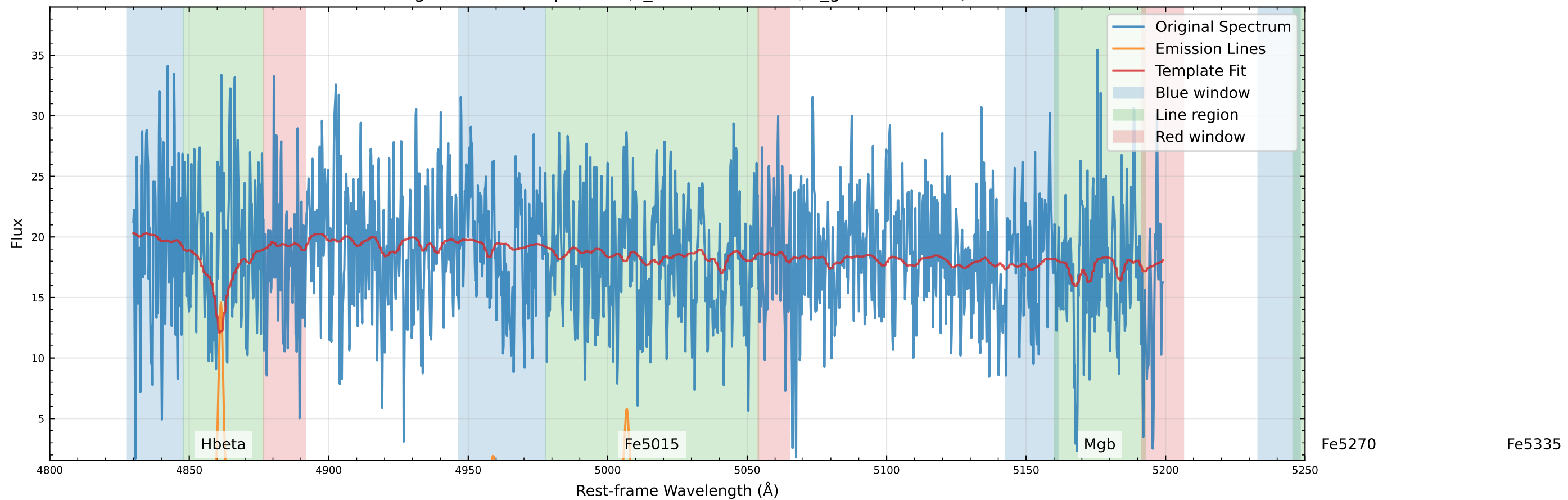
Original Data Comparison (v_star=-26.0 km/s, v_gas=-8.6 km/s)
