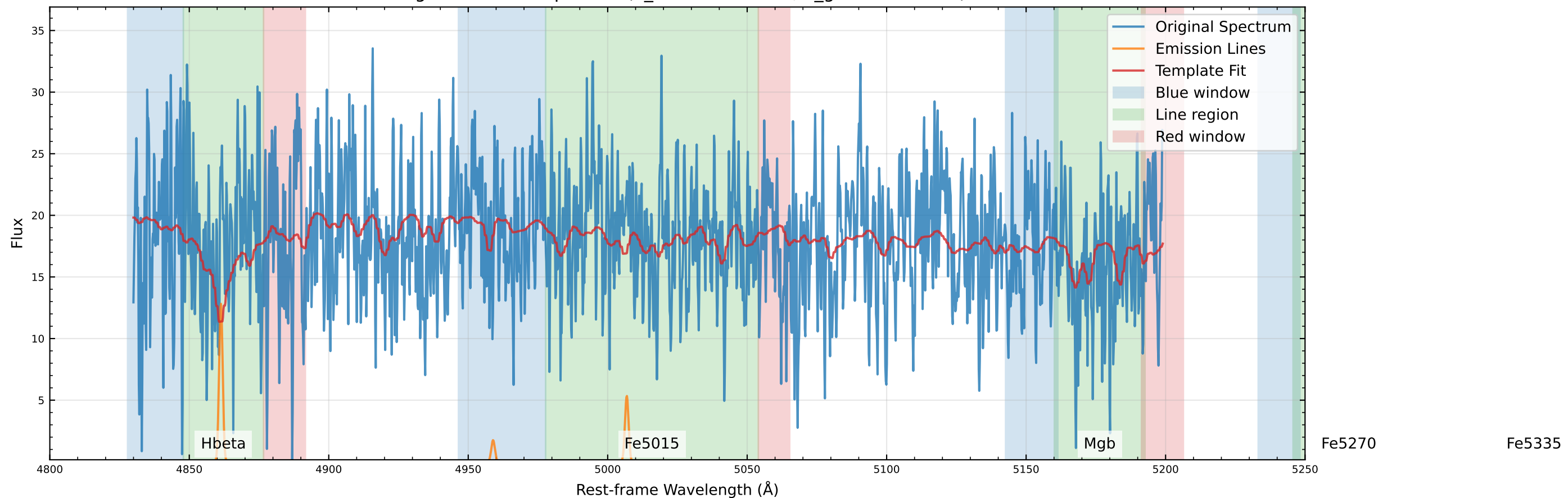
Original Data Comparison (v_star=20.0 km/s, v_gas=23.4 km/s)
