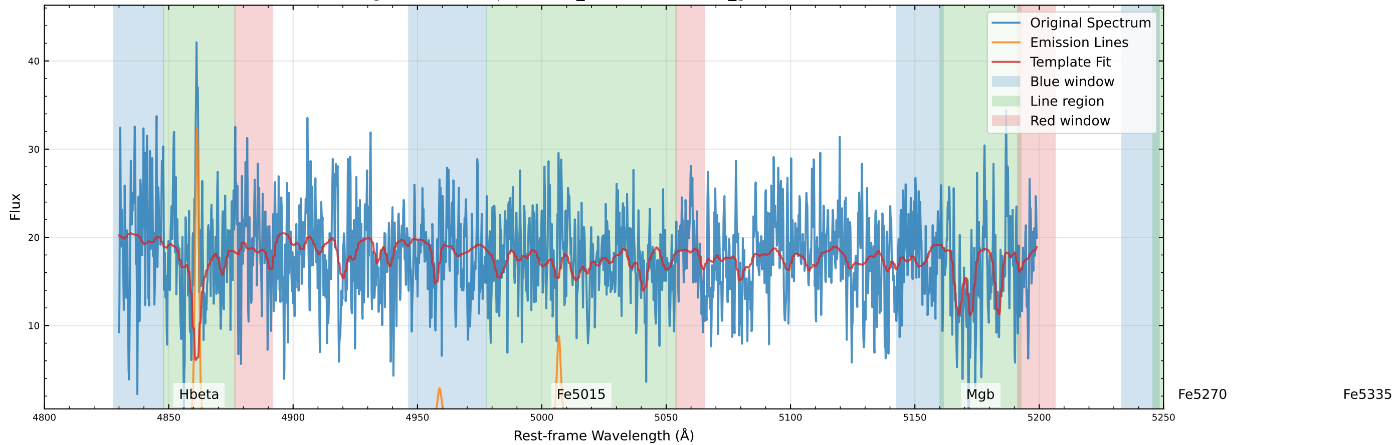
Original Data Comparison (v_star=14.5 km/s, v_gas=-0.6 km/s)
