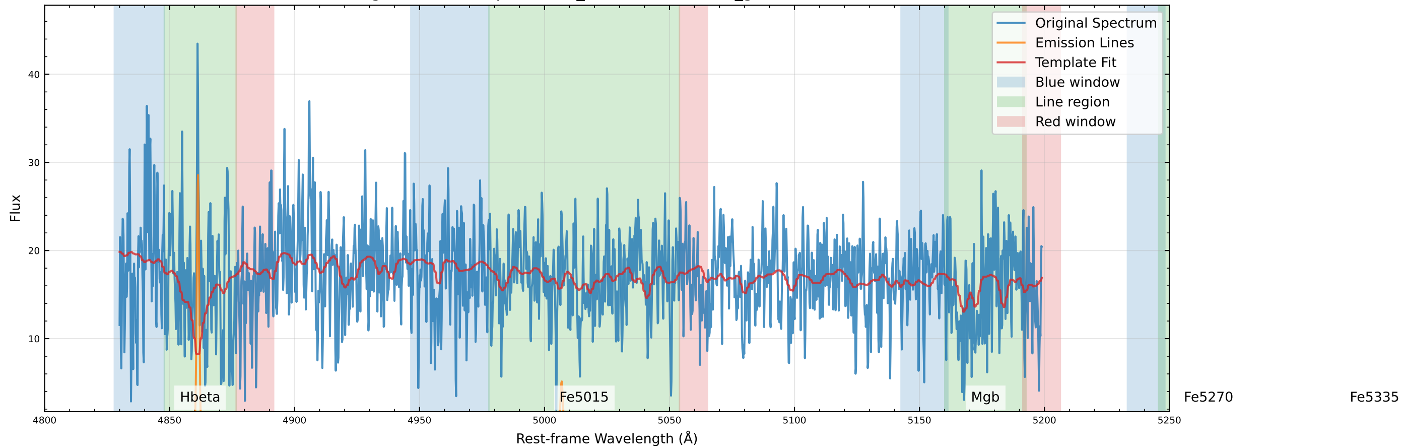
Original Data Comparison (v_star=-15.2 km/s, v_gas=-3.9 km/s)
