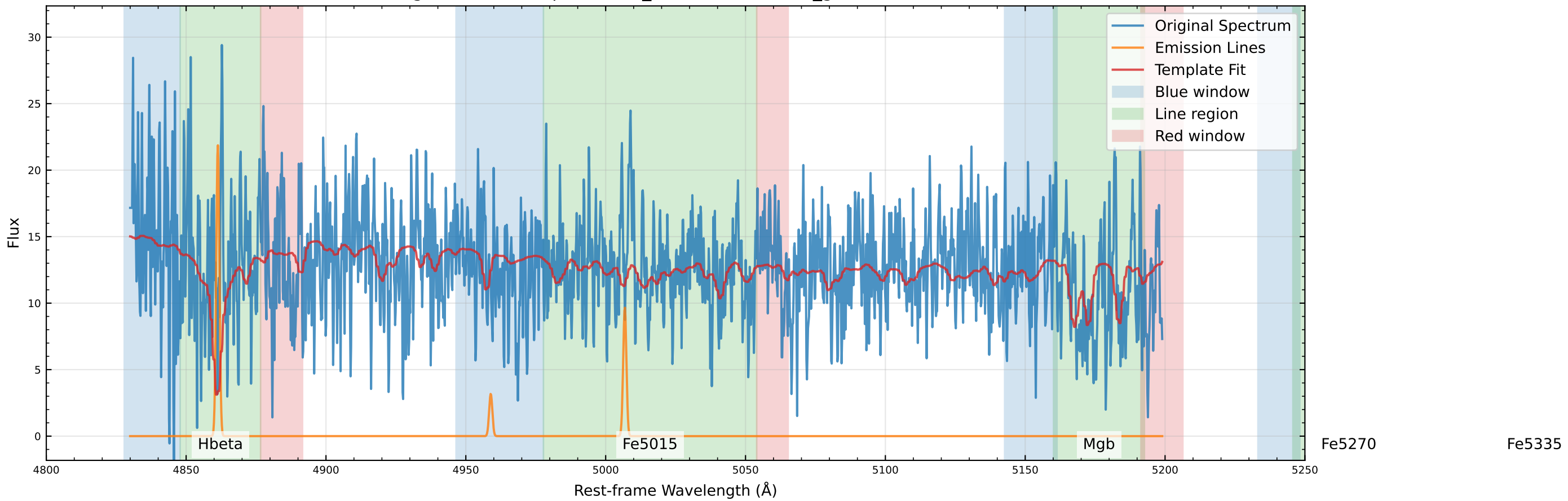
Original Data Comparison (v_star=94.1 km/s, v_gas=91.4 km/s)
