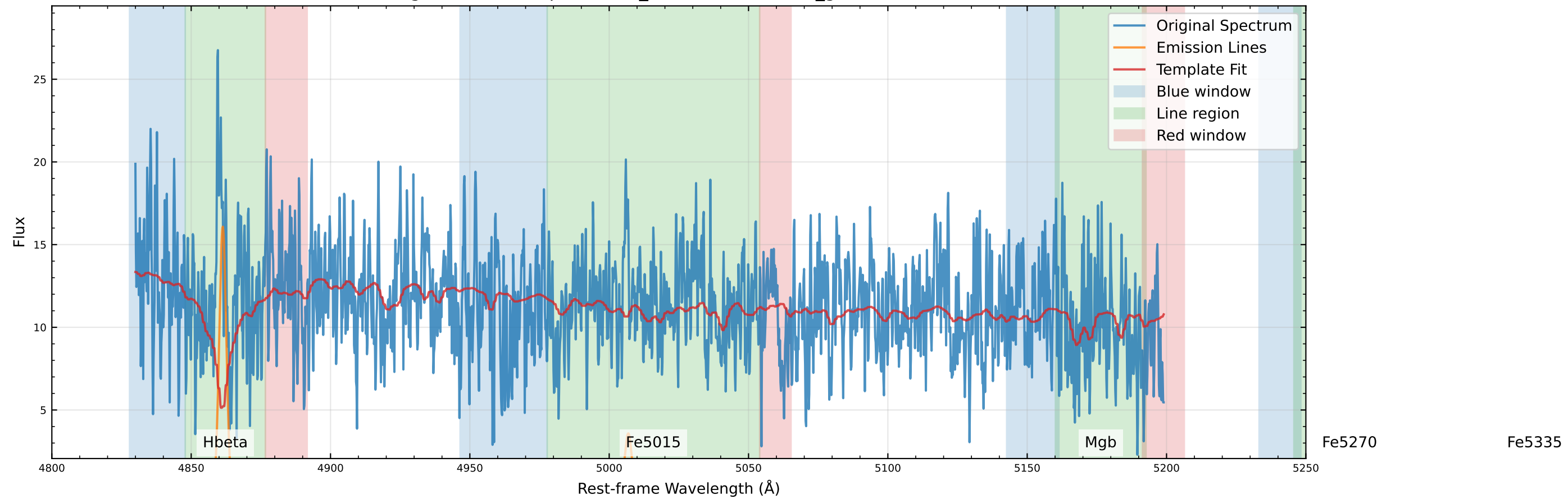
Original Data Comparison (v_star=-70.6 km/s, v_gas=-66.6 km/s)
