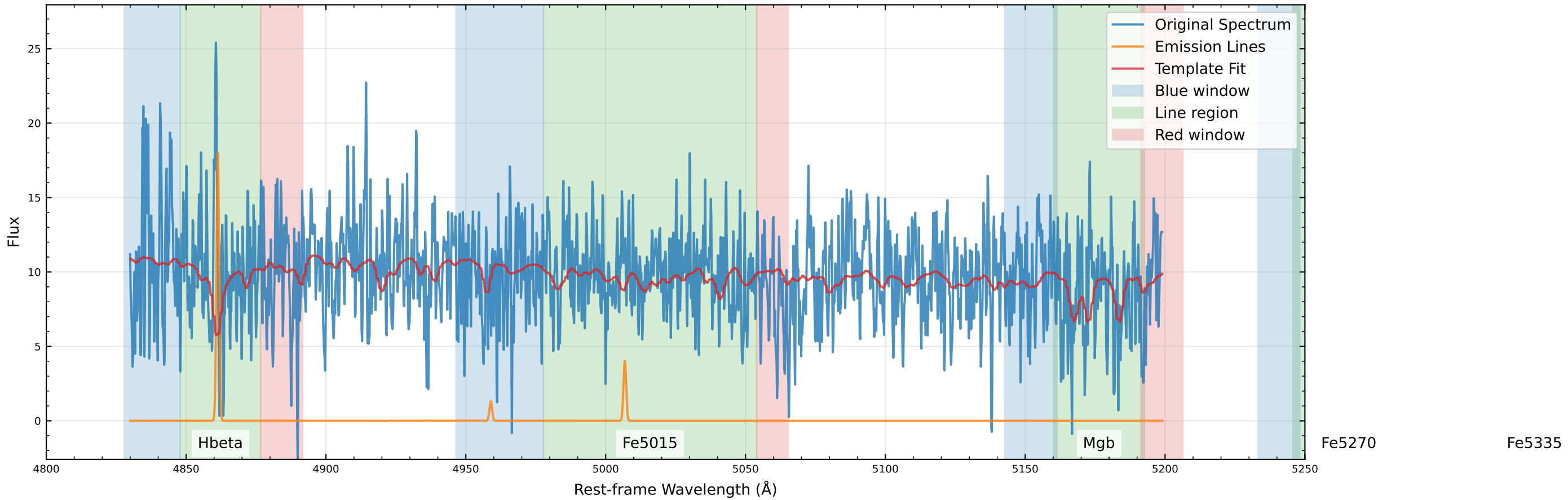
Original Data Comparison (v_star=-74.1 km/s, v_gas=-50.3 km/s)
