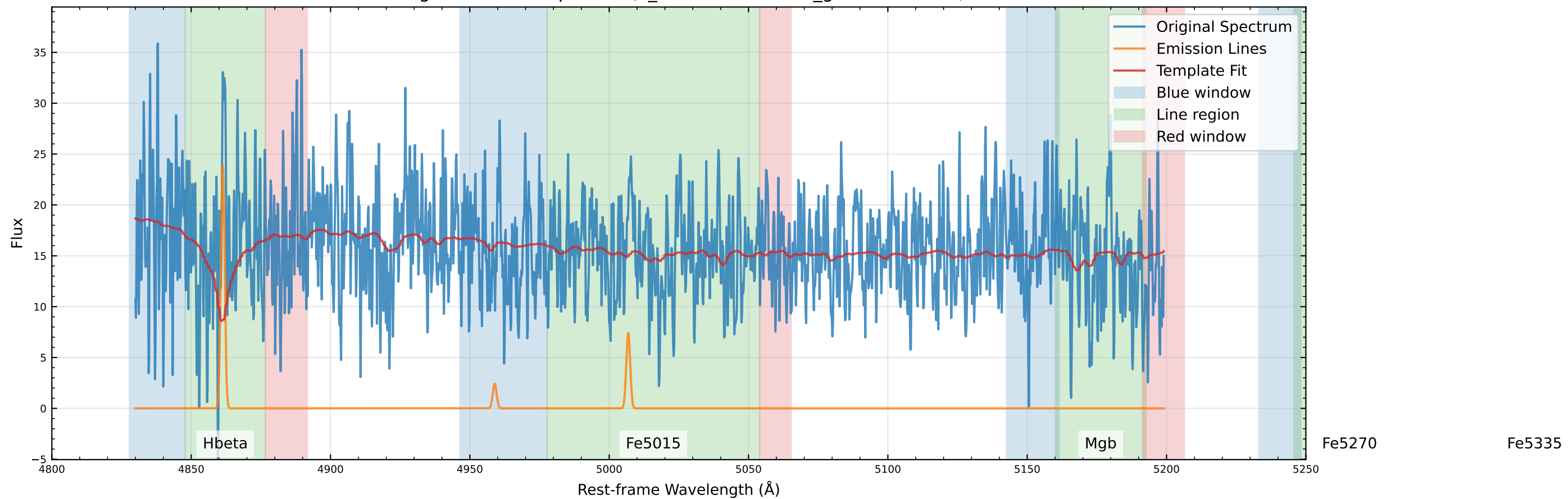
Original Data Comparison (v_star=-7.7 km/s, v_gas=25.5 km/s)
