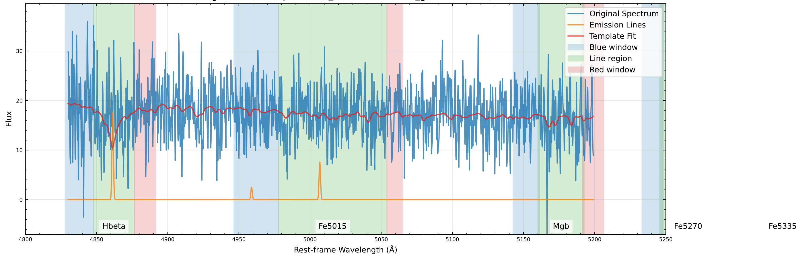
Original Data Comparison (v_star=30.3 km/s, v_gas=49.5 km/s)
