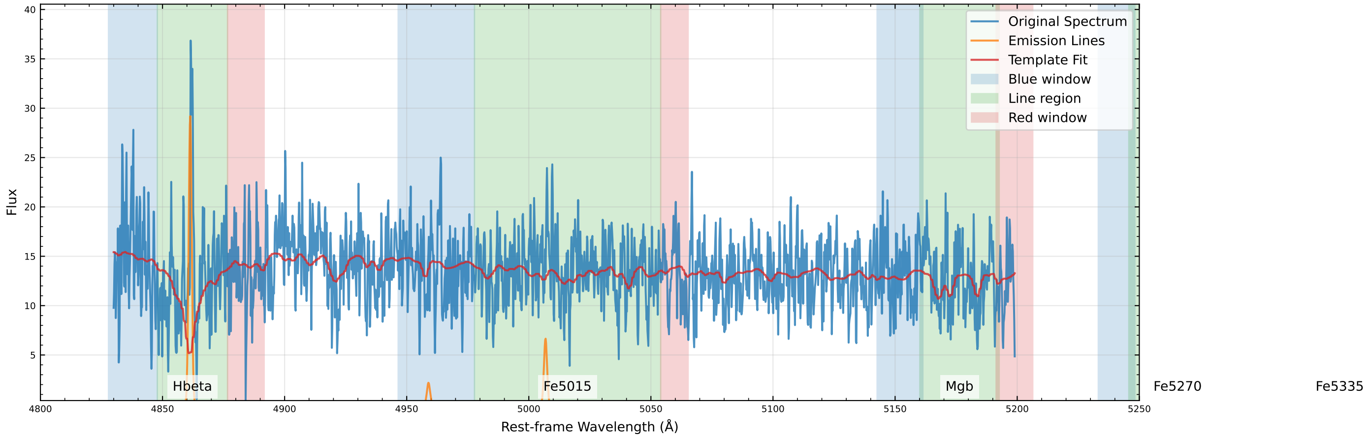
Original Data Comparison (v_star=10.5 km/s, v_gas=35.6 km/s)
