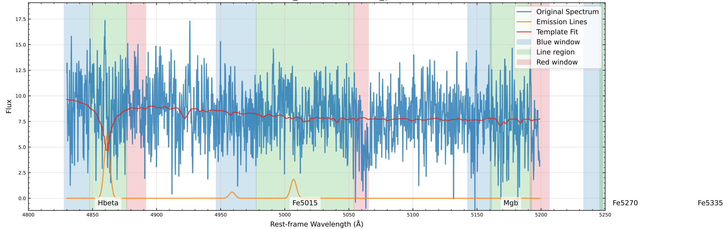
Original Data Comparison (v_star=-219.7 km/s, v_gas=-174.1 km/s)
