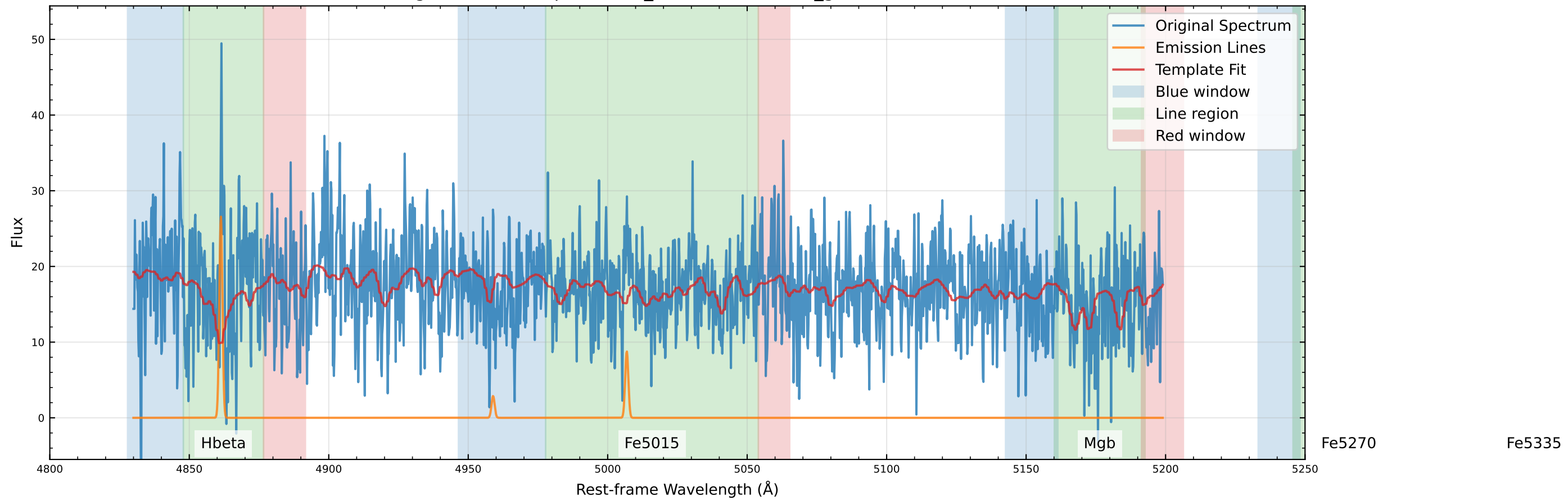
Original Data Comparison (v_star=45.4 km/s, v_gas=19.0 km/s)
