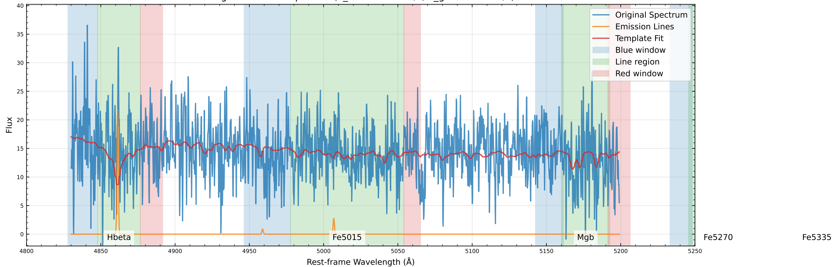
Original Data Comparison (v_star=20.3 km/s, v_gas=28.2 km/s)
