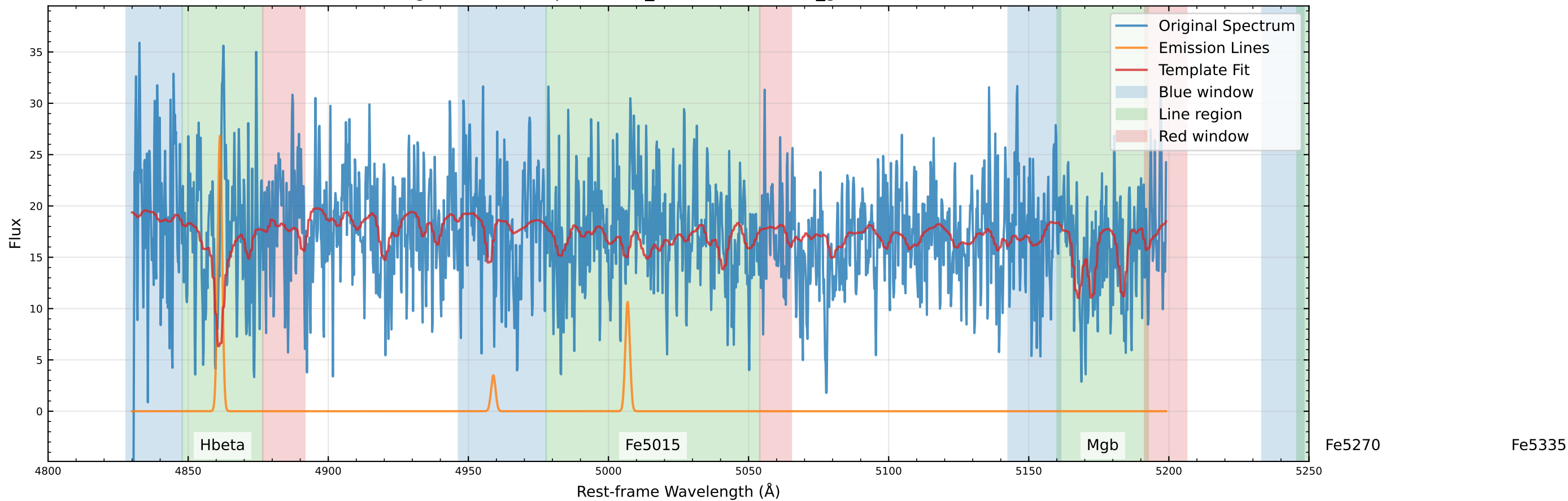
Original Data Comparison (v_star=73.4 km/s, v_gas=72.4 km/s)
