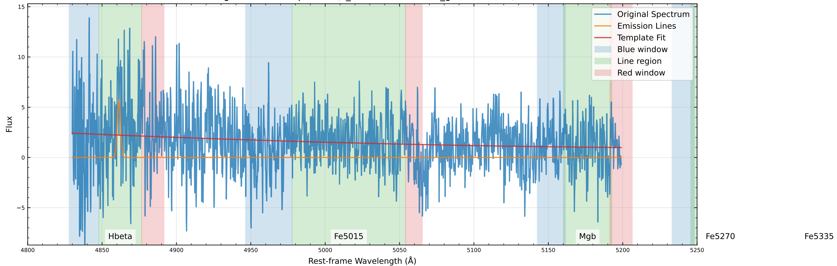
Original Data Comparison (v_star=-95.4 km/s, v_gas=5.1 km/s)
