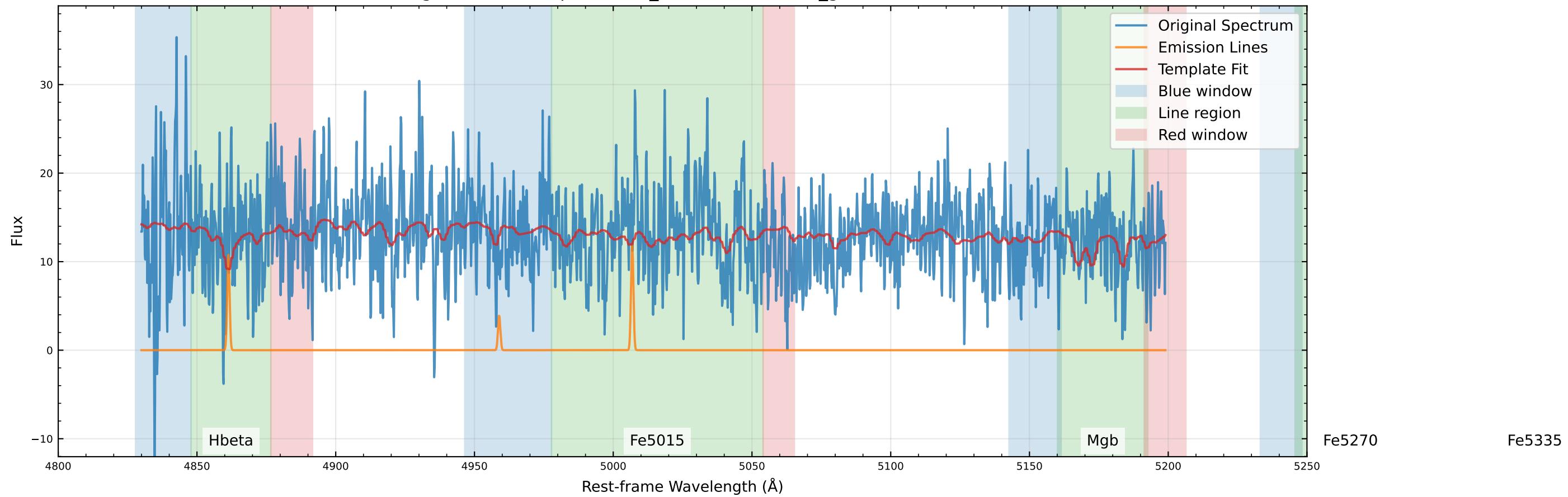
Original Data Comparison (v_star=26.9 km/s, v_gas=65.3 km/s)
