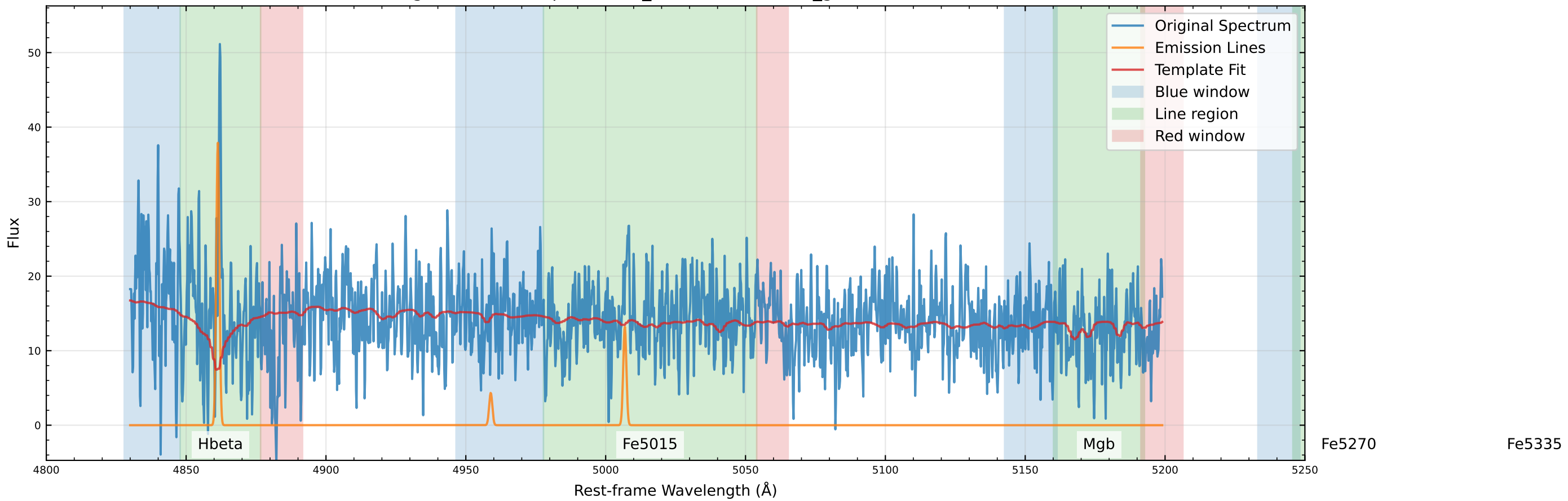
Original Data Comparison (v_star=47.0 km/s, v_gas=46.7 km/s)
