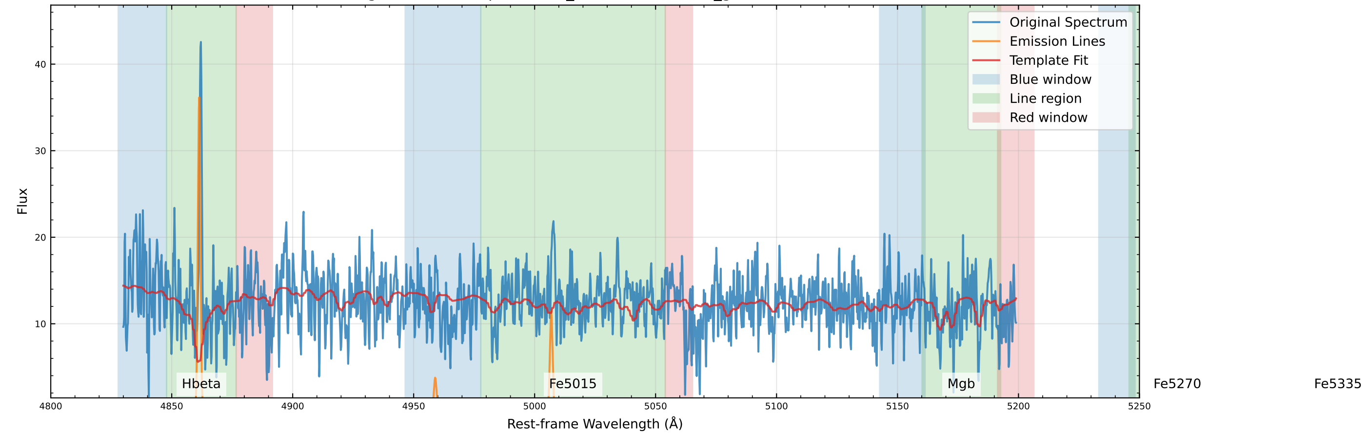
Original Data Comparison (v_star=38.4 km/s, v_gas=37.2 km/s)
