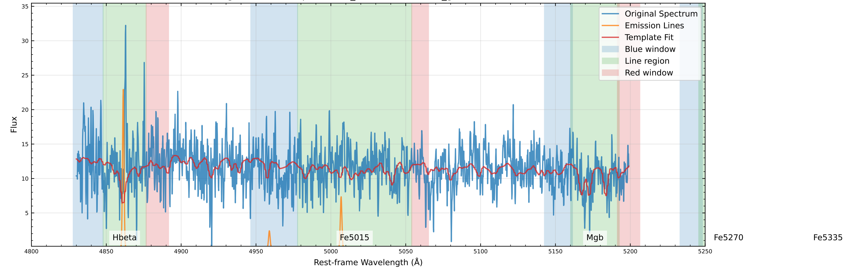
Original Data Comparison (v_star=75.9 km/s, v_gas=87.0 km/s)
