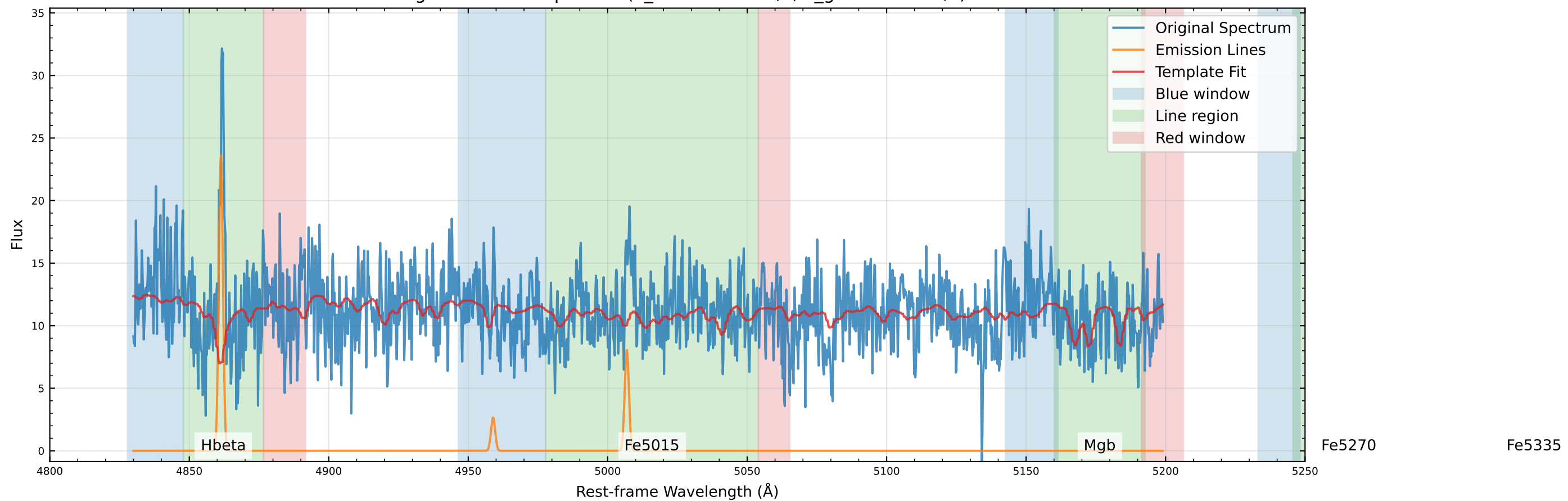
Original Data Comparison (v_star=22.0 km/s, v_gas=28.2 km/s)
