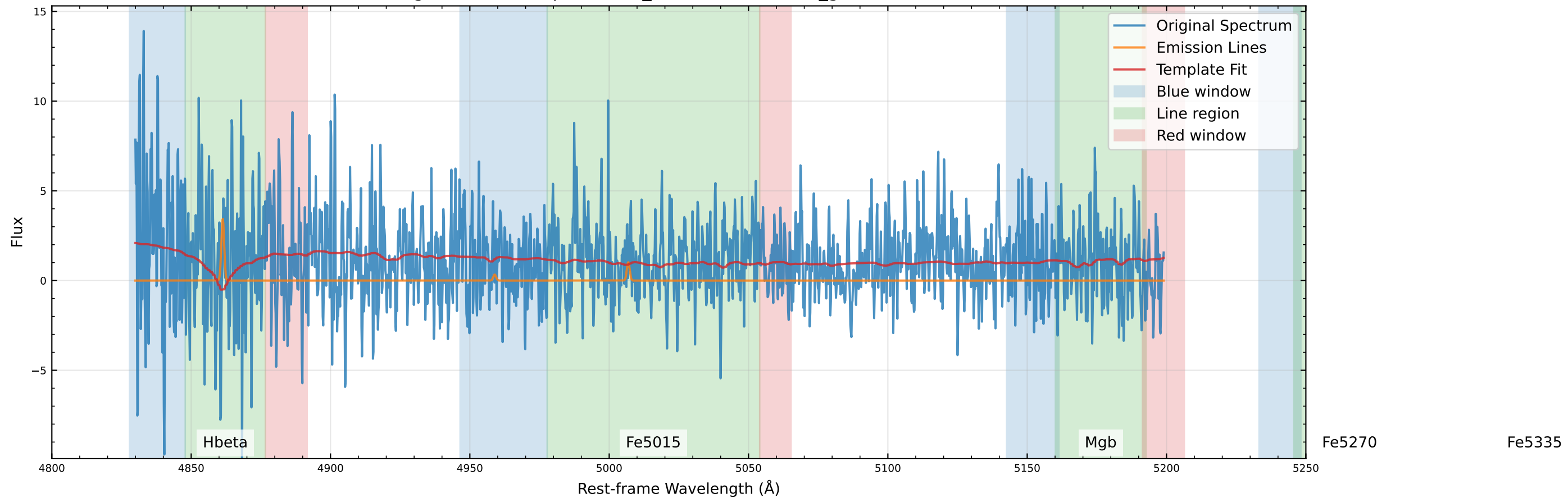
Original Data Comparison (v_star=-28.6 km/s, v_gas=34.8 km/s)
