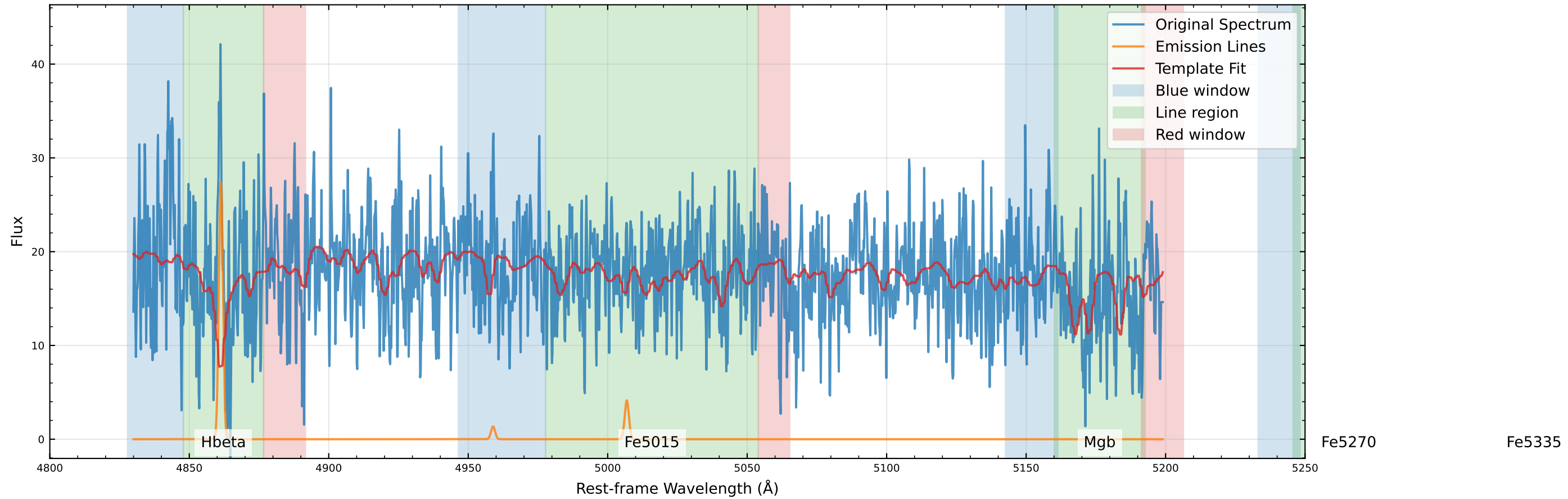
Original Data Comparison (v_star=-68.7 km/s, v_gas=-28.3 km/s)
