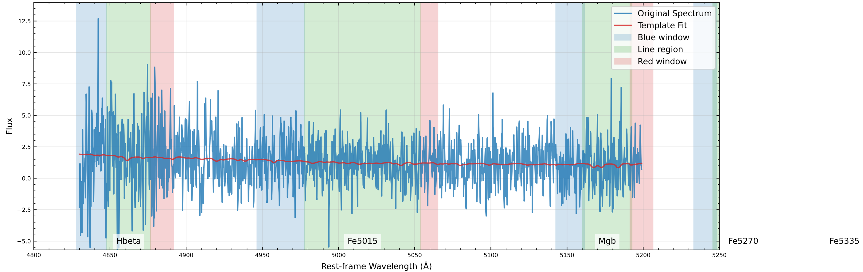
Original Data Comparison (v_star=-9.1 km/s)
