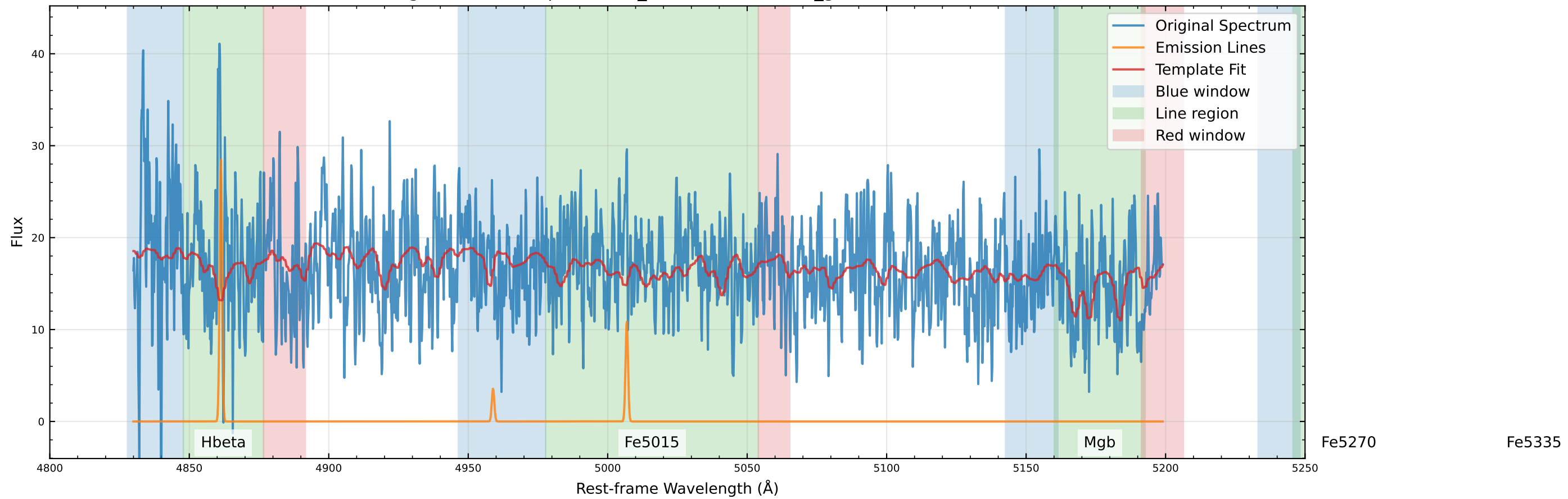
Original Data Comparison (v_star=-59.1 km/s, v_gas=-38.3 km/s)
