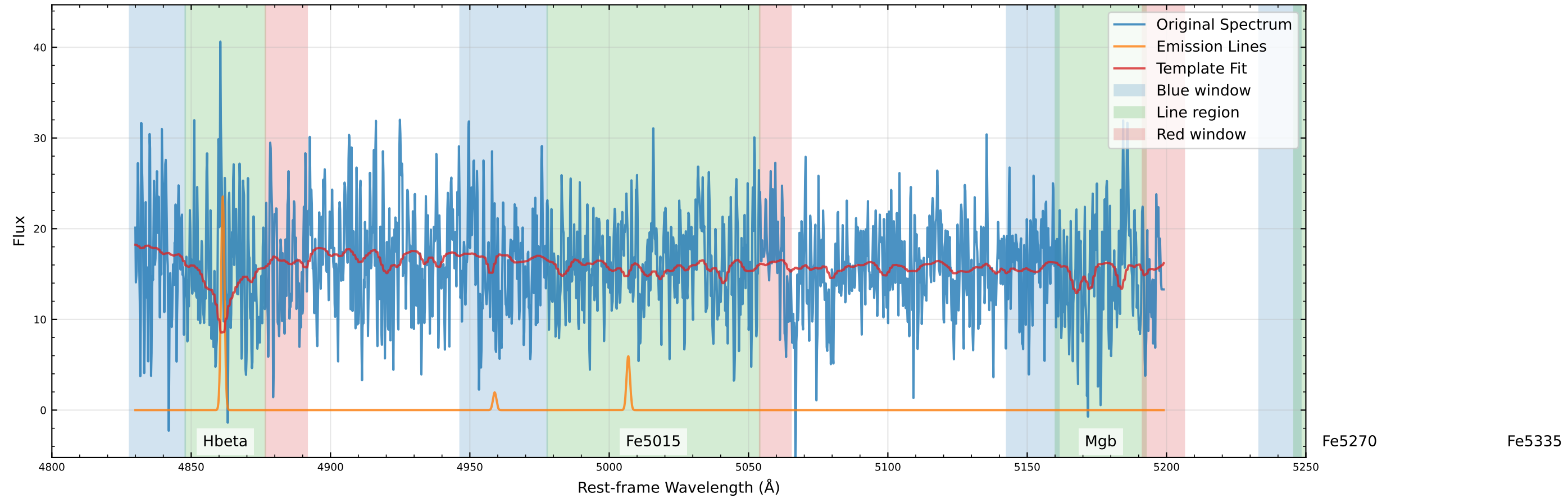
Original Data Comparison (v_star=-88.0 km/s, v_gas=-56.3 km/s)
