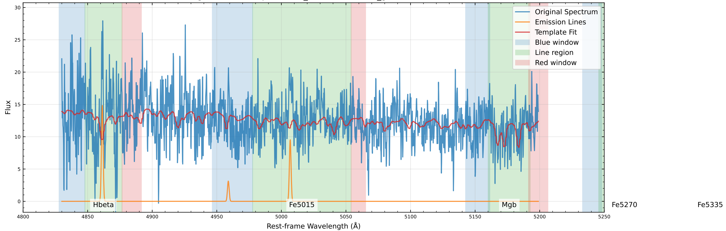
Original Data Comparison (v_star=4.2 km/s, v_gas=2.8 km/s)
