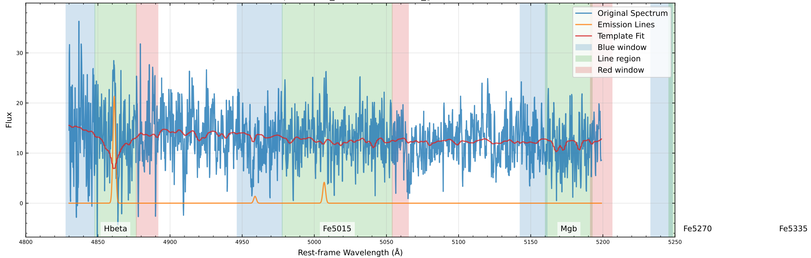
Original Data Comparison (v_star=-30.4 km/s, v_gas=-14.7 km/s)
