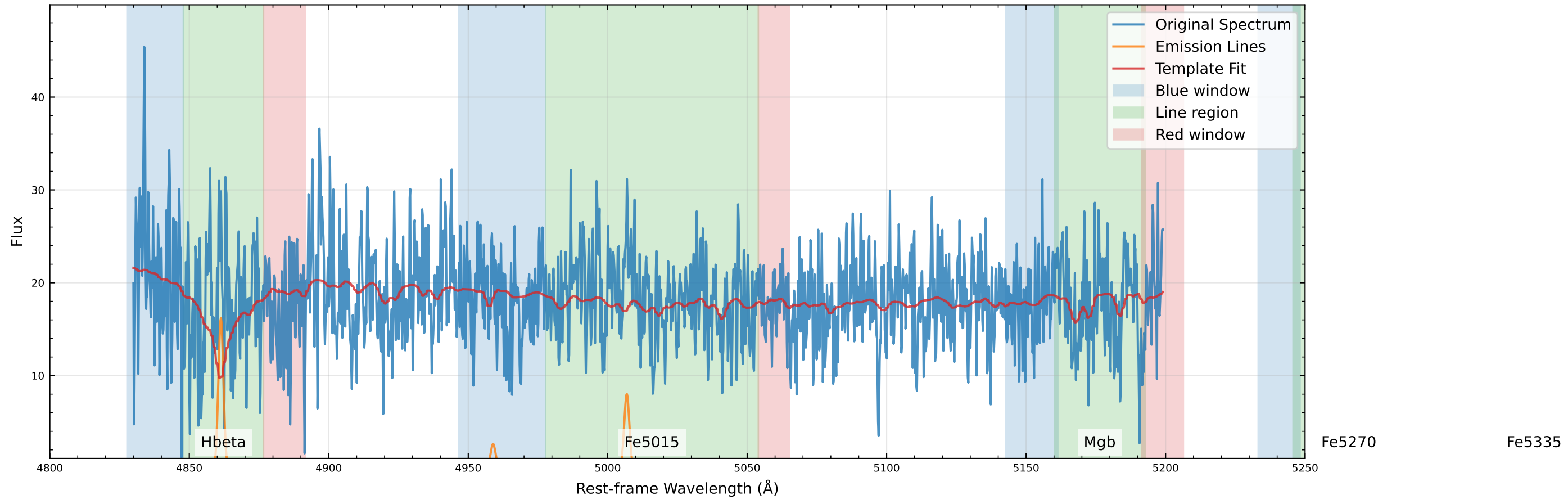
Original Data Comparison (v_star=-36.9 km/s, v_gas=-17.6 km/s)
