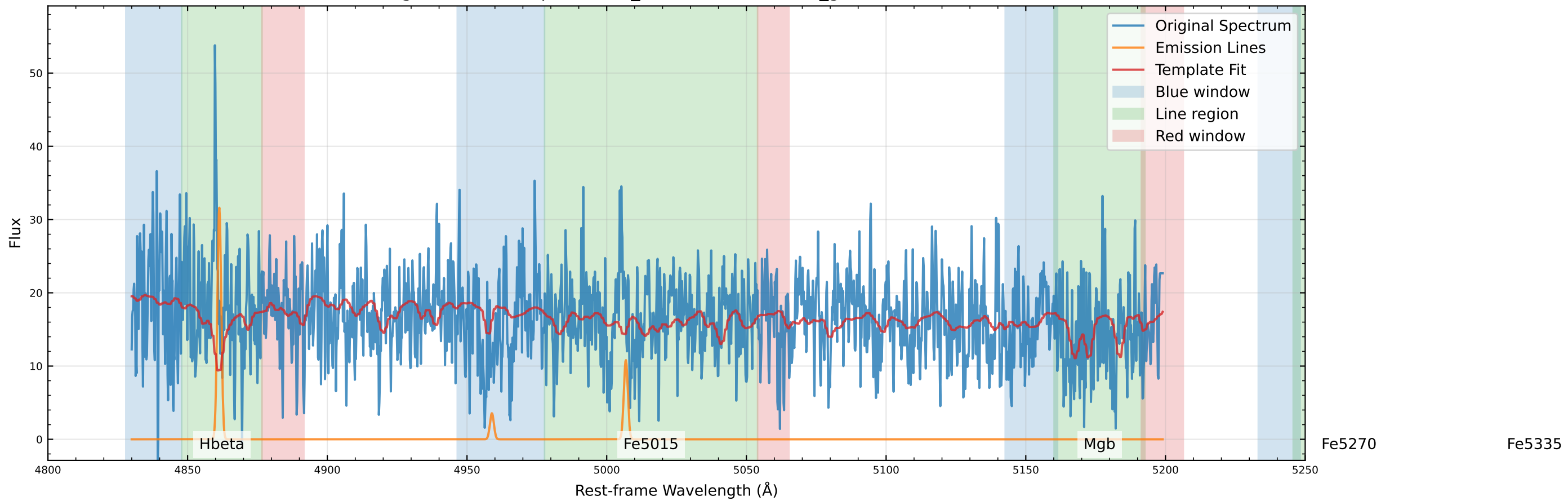
Original Data Comparison (v_star=-111.6 km/s, v_gas=-93.7 km/s)
