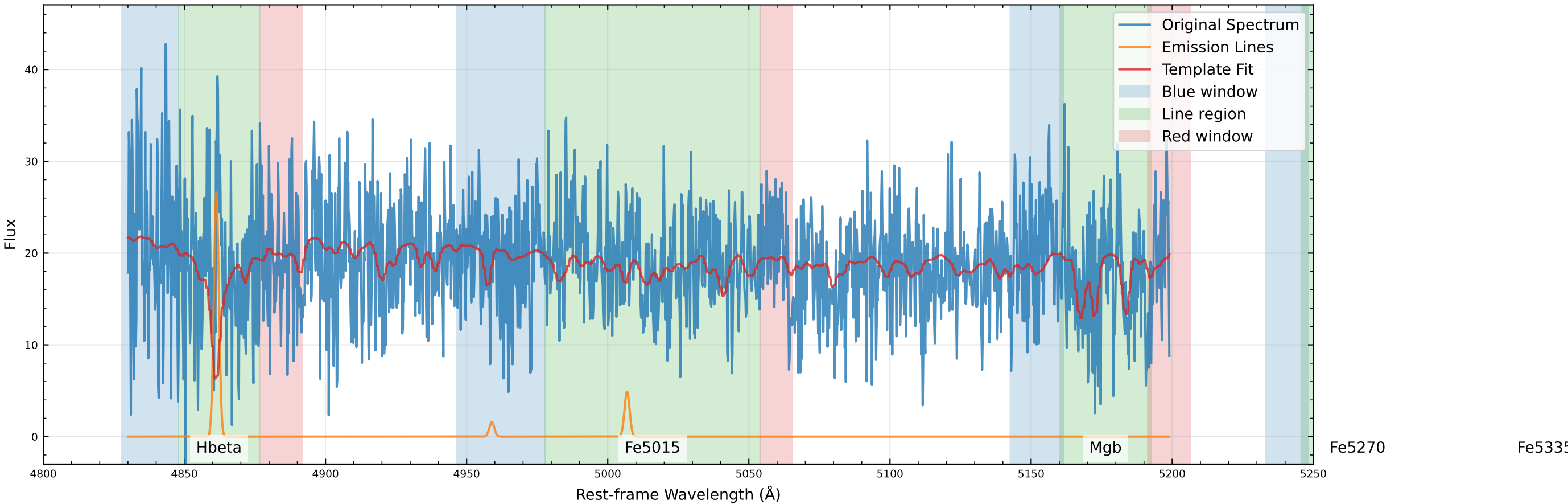
Original Data Comparison (v_star=19.9 km/s, v_gas=36.1 km/s)
