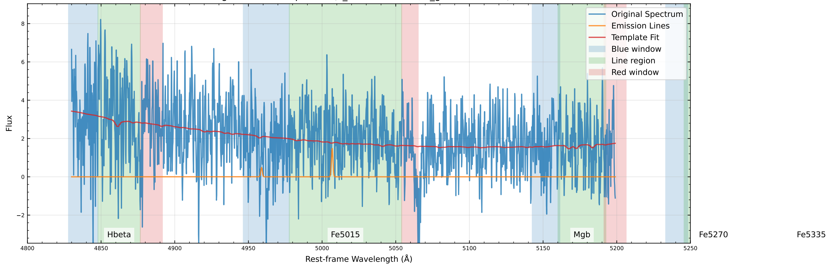
Original Data Comparison (v_star=-0.4 km/s, v_gas=34.3 km/s)
