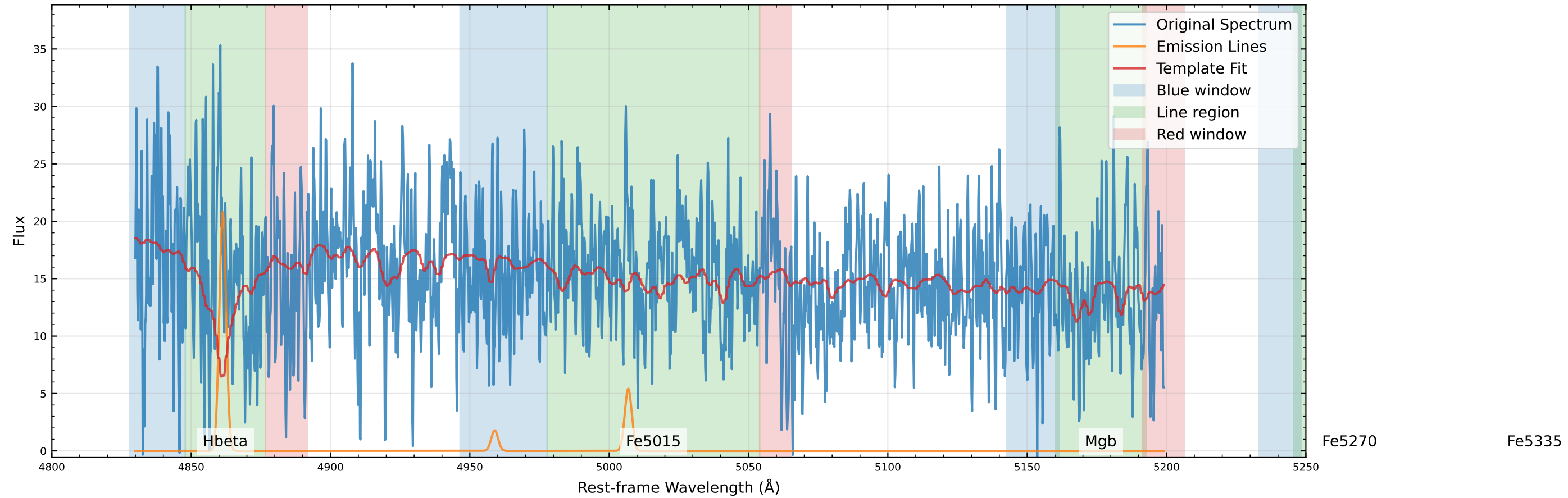
Original Data Comparison (v_star=-32.3 km/s, v_gas=-62.8 km/s)
