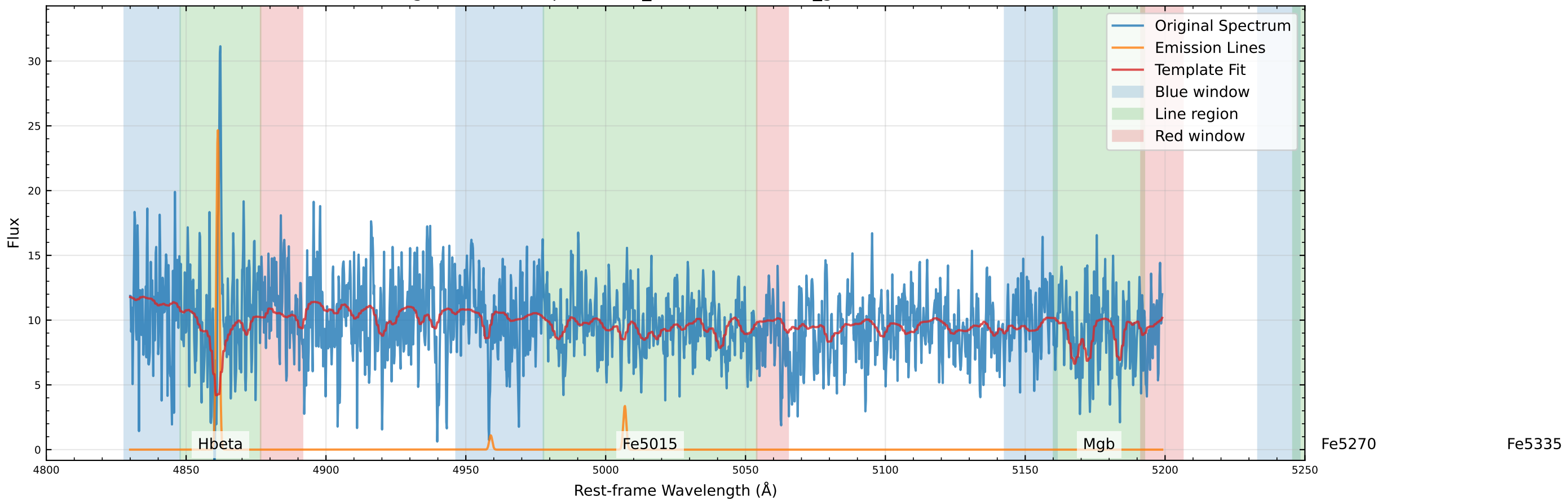
Original Data Comparison (v_star=56.7 km/s, v_gas=46.5 km/s)
