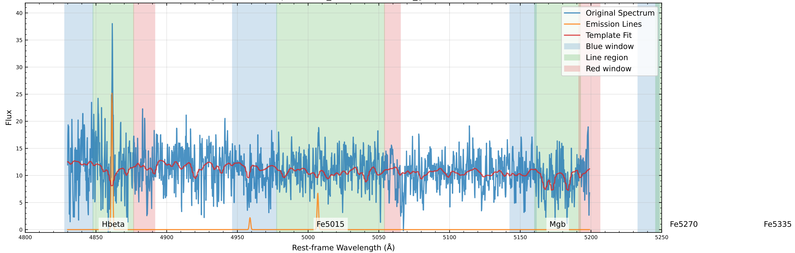
Original Data Comparison (v_star=23.4 km/s, v_gas=15.1 km/s)
