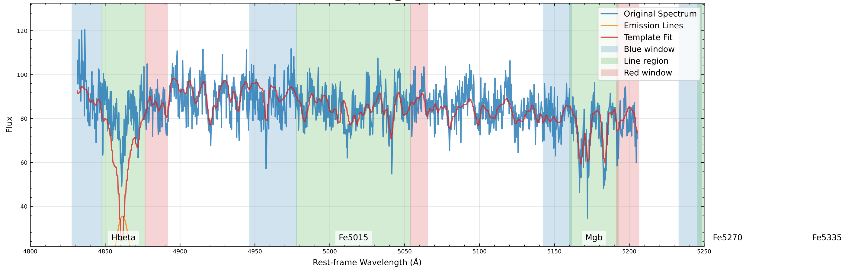
Original Data Comparison (v_star=-5.6 km/s)
