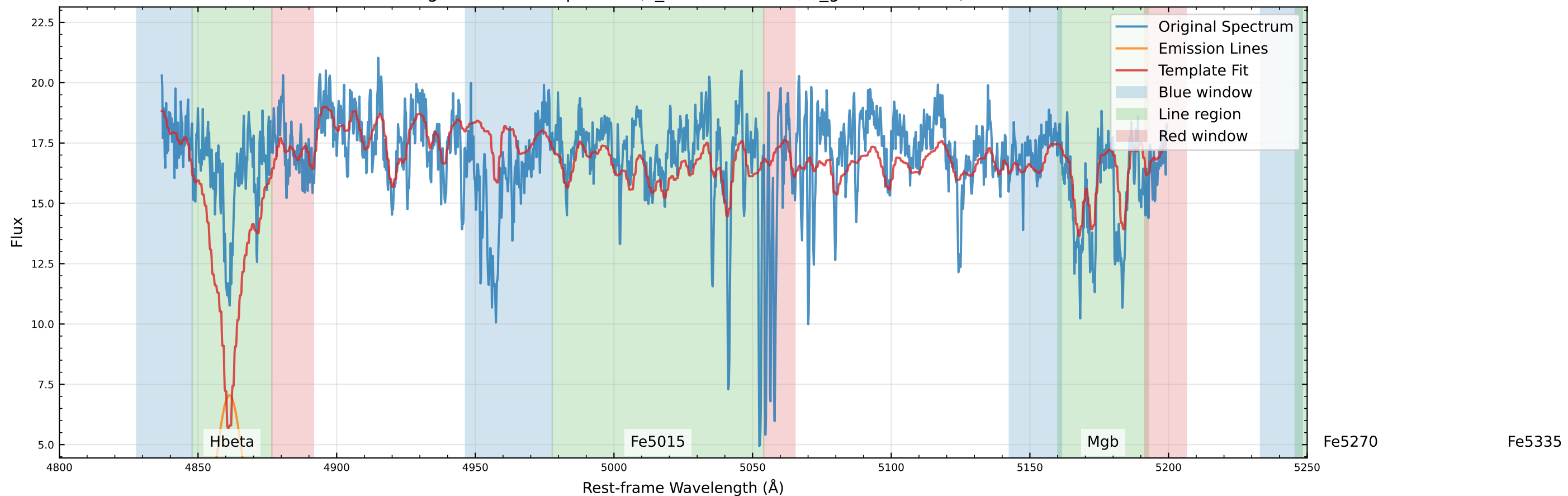
Original Data Comparison (v_star=-9.0 km/s, v_gas=-0.4 km/s)
