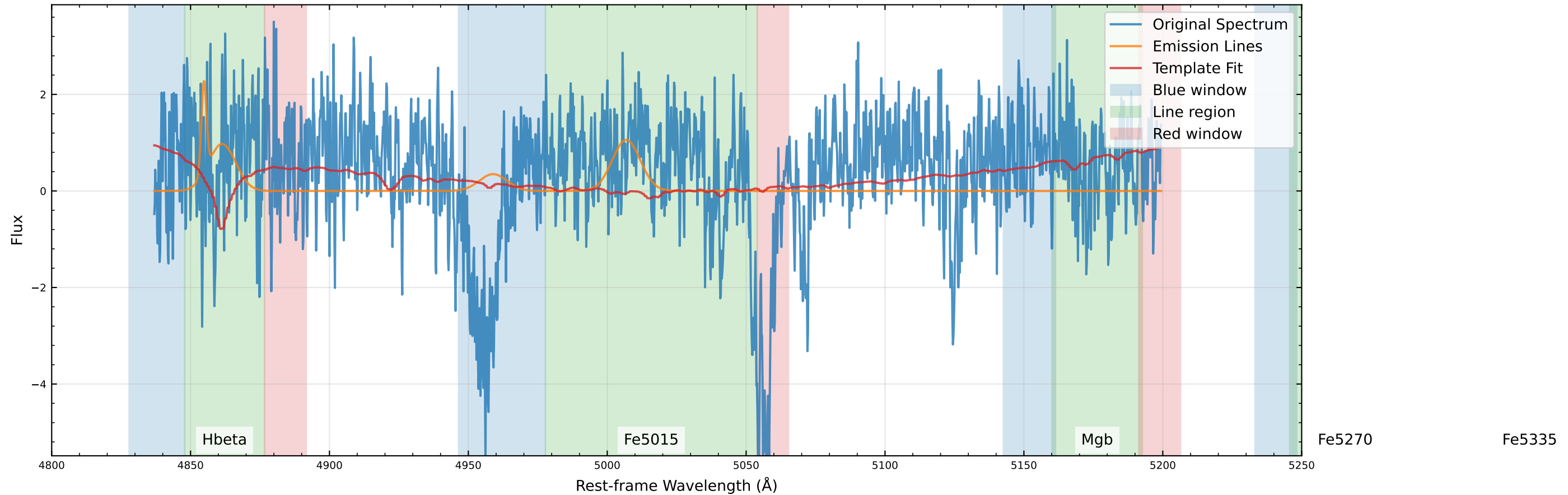
Original Data Comparison (v_star=130.4 km/s, v_gas=430.4 km/s)
