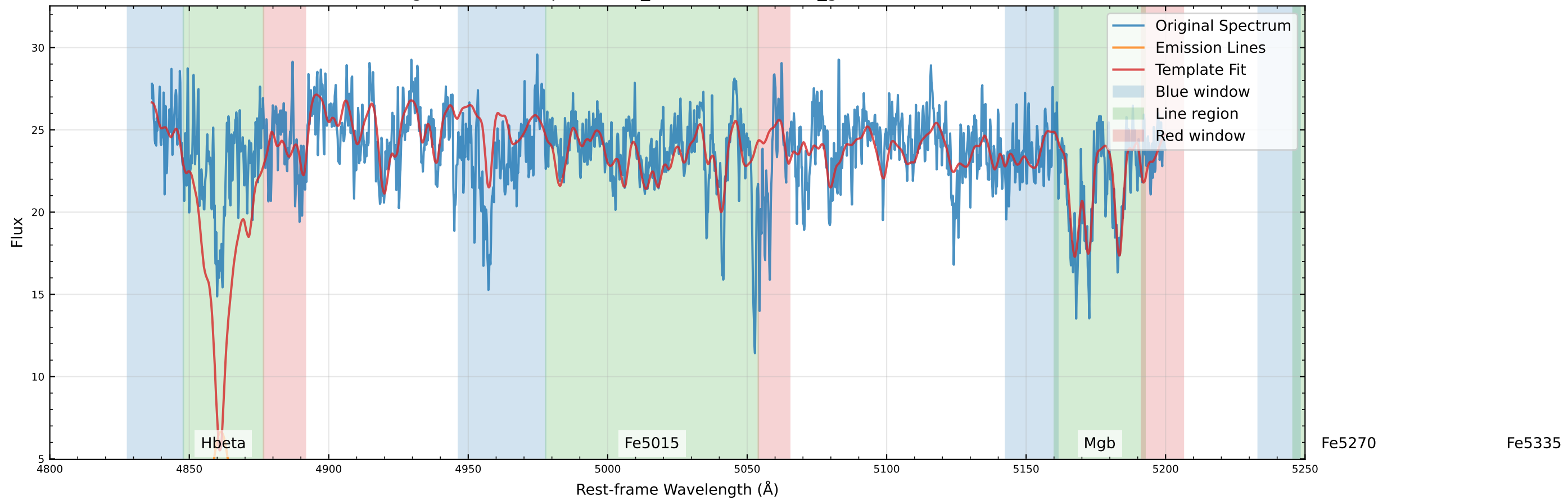
Original Data Comparison (v_star=-12.7 km/s, v_gas=59.3 km/s)
