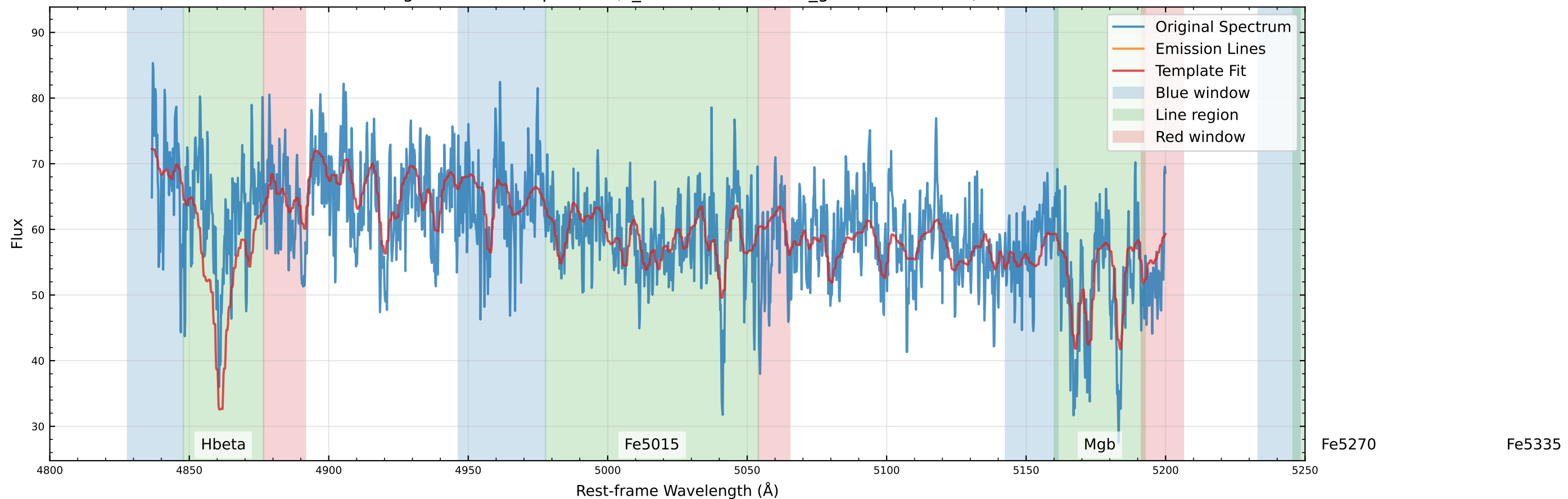
Original Data Comparison ( v_{\text{star}}=-15.3 km/s, v_{\text{gas}}=-123.7 km/s)
