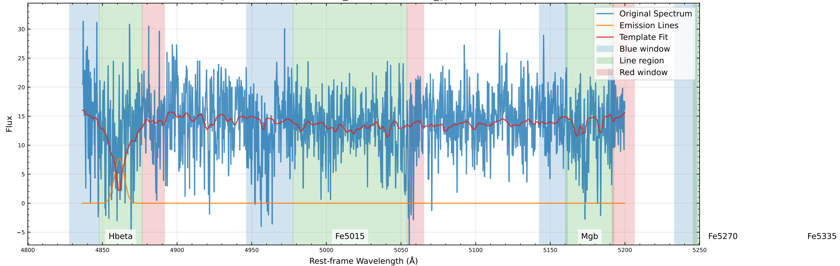
Original Data Comparison (v_star=40.9 km/s, v_gas=146.5 km/s)
