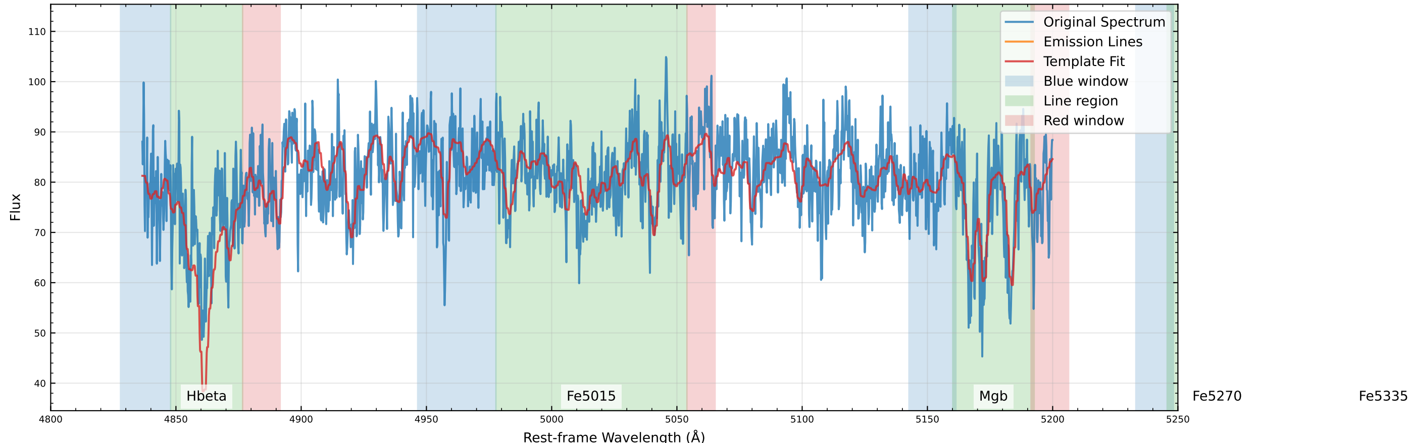
Original Data Comparison (v_star=-22.6 km/s, v_gas=7.7 km/s)
