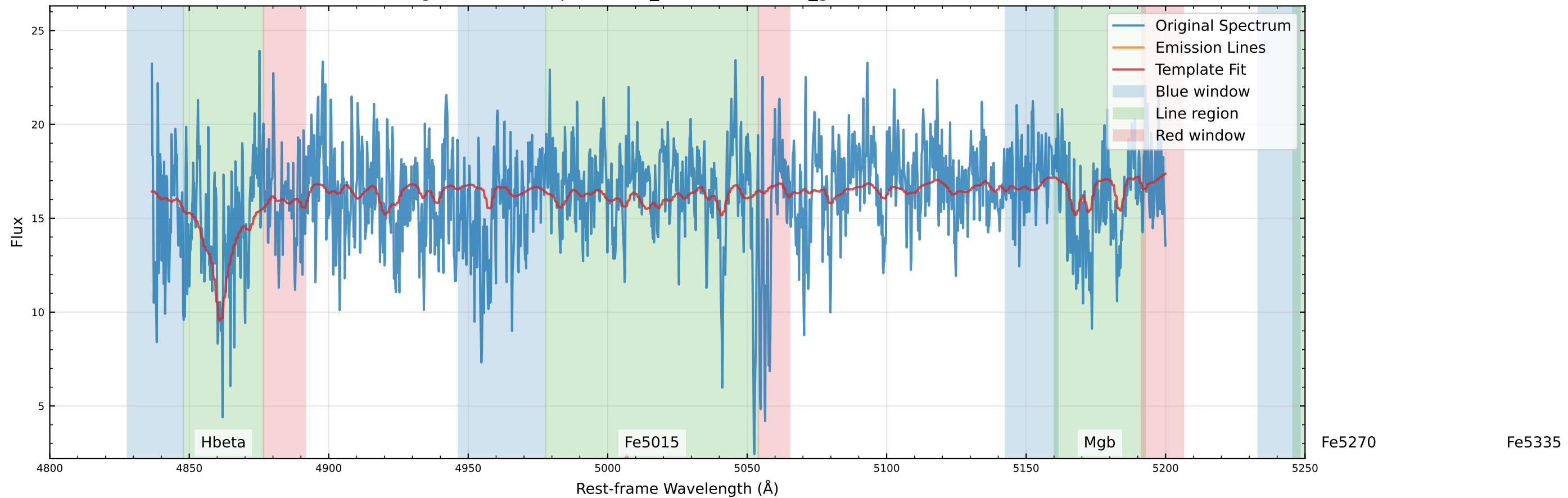
Original Data Comparison (v_star=3.6 km/s, v_gas=76.7 km/s)
