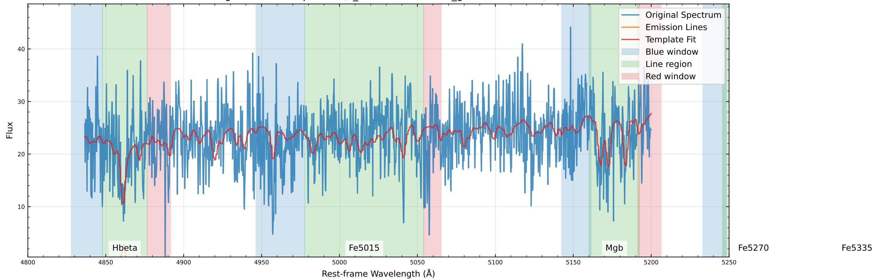
Original Data Comparison (v_star=-44.0 km/s, v_gas=-108.9 km/s)
