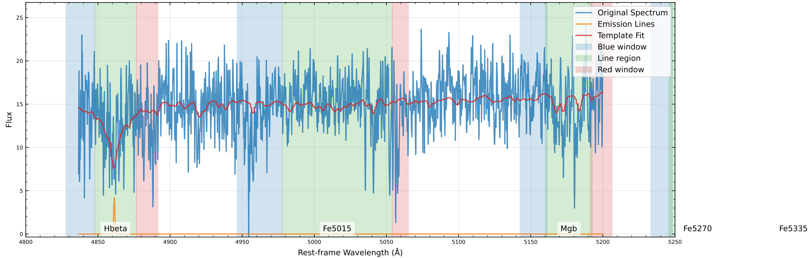
Original Data Comparison (v_star=-19.0 km/s, v_gas=-45.6 km/s)
