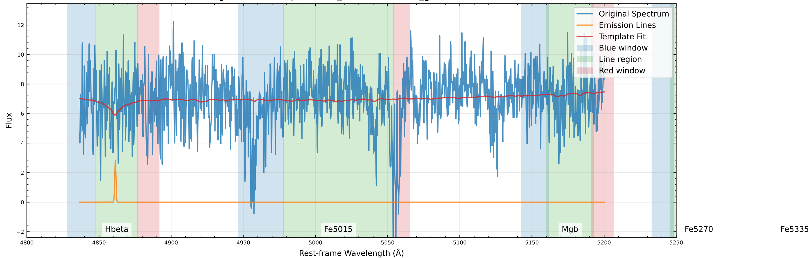
Original Data Comparison (v_star=8.4 km/s, v_gas=10.0 km/s)
