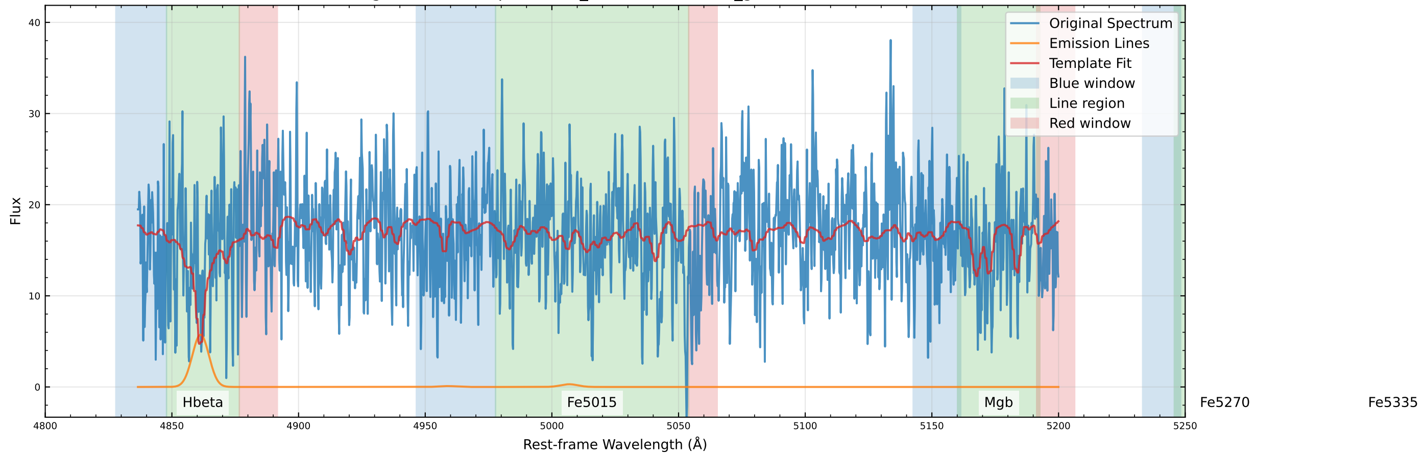
Original Data Comparison ( v_{\text{star}}=51.7 km/s, v_{\text{gas}}=171.5 km/s)
