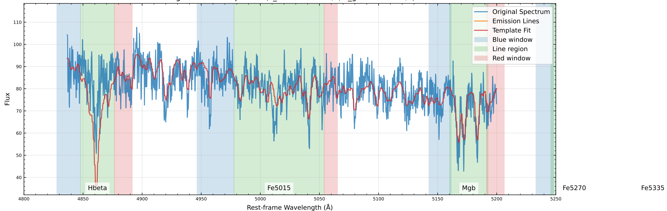
Original Data Comparison (v_star=-15.5 km/s, v_gas=-19.0 km/s)
