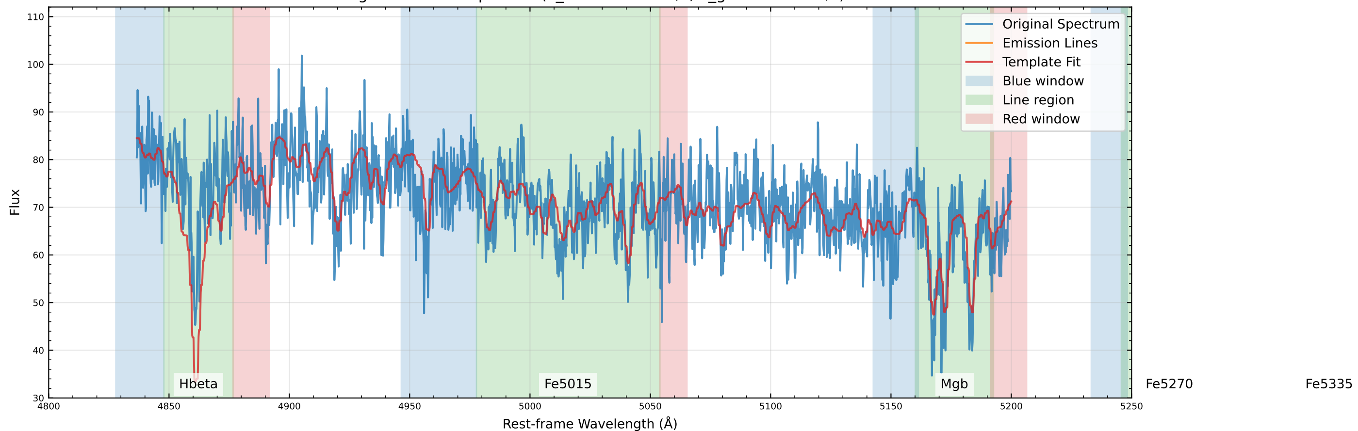
Original Data Comparison (v_star=-21.5 km/s, v_gas=-51.8 km/s)
