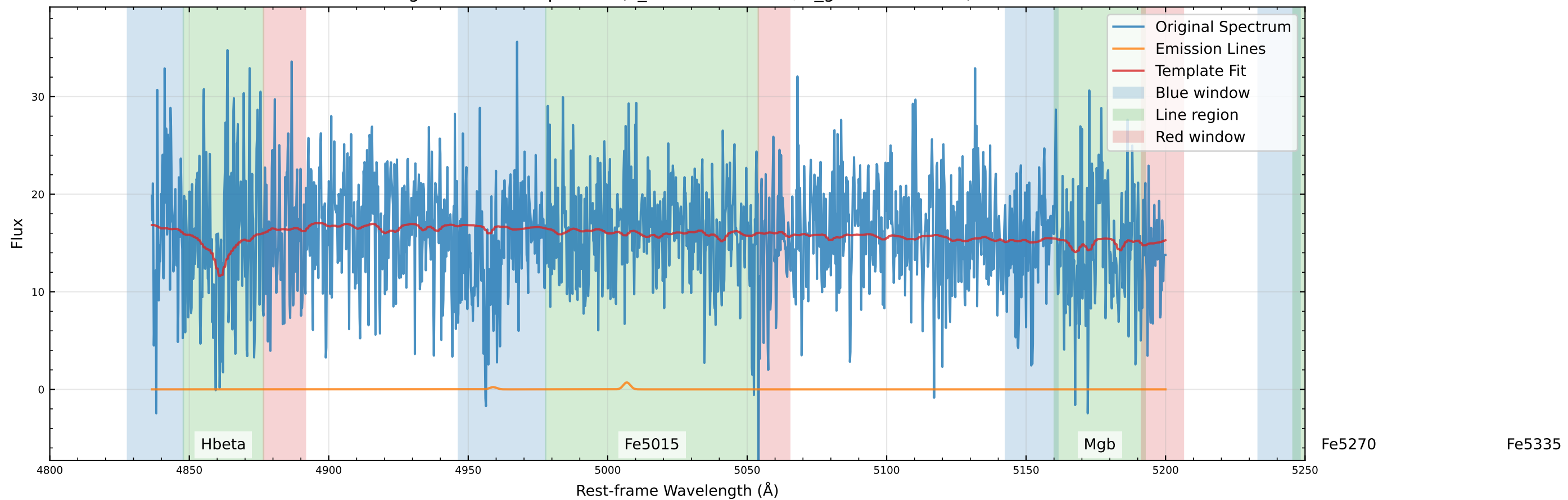
Original Data Comparison (v_star=-64.3 km/s, v_gas=-54.2 km/s)
