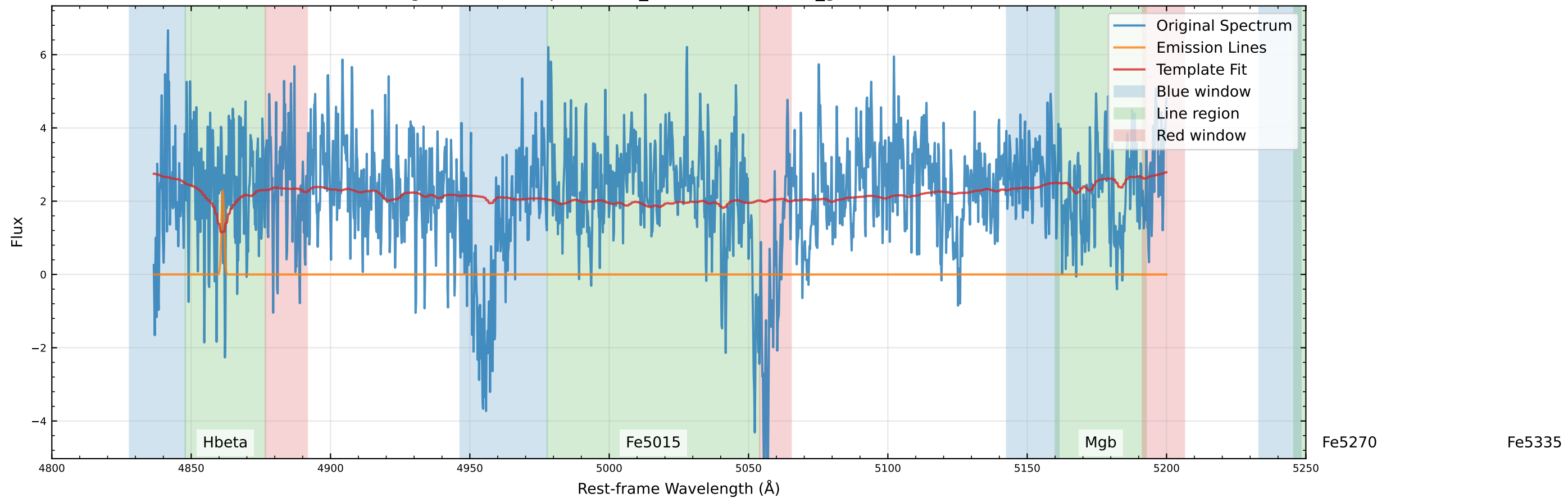
Original Data Comparison (v_star=-23.3 km/s, v_gas=-51.6 km/s)
